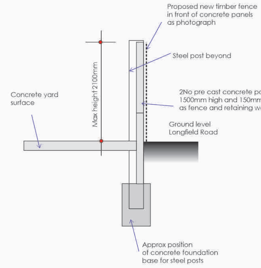
Typical Section - 1:50 Front boundary with Longfield Road
