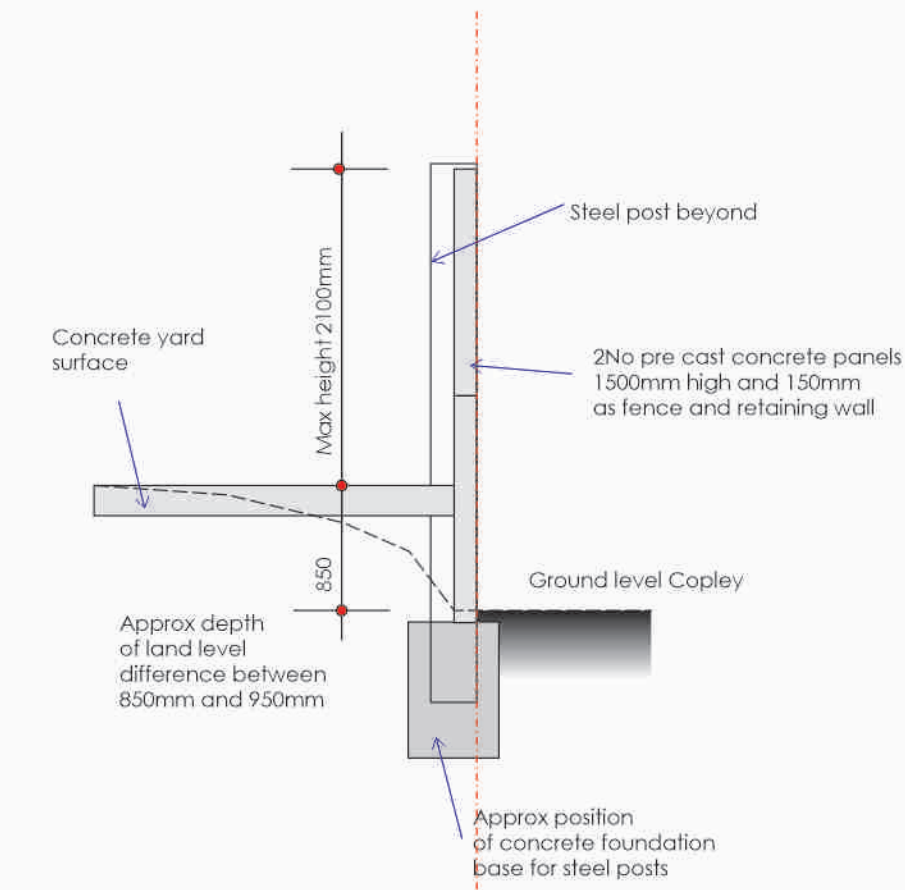
Typical Section - 1:50 Side boundary with Copley
