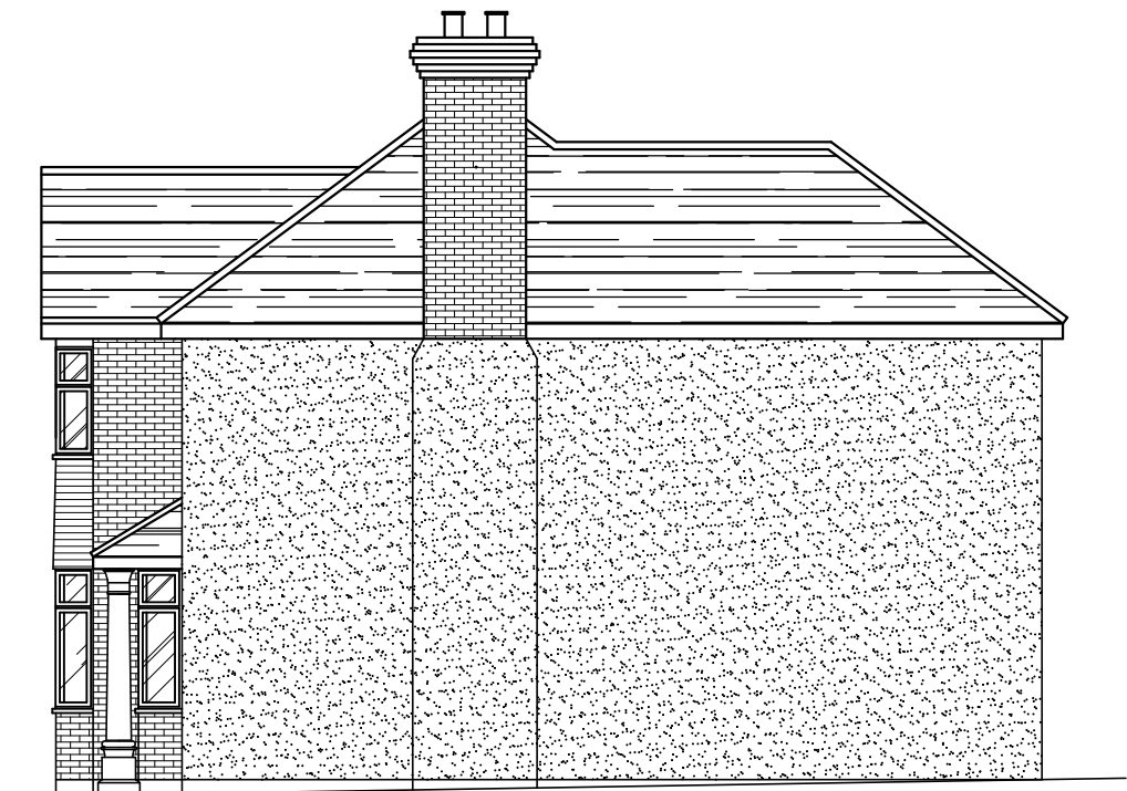
Existing Side (South) Elevation Scale 1:100 @ A1
