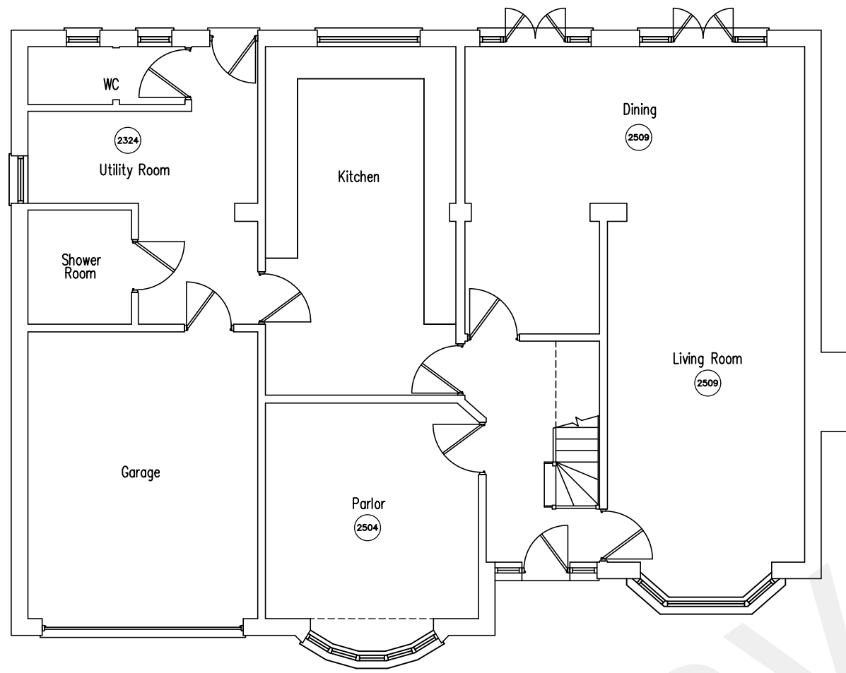
Existing Ground Floor Plan Scale 1:100 @ A1
