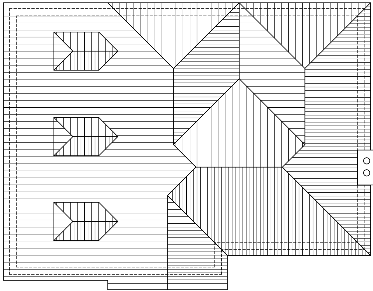
Existing Roof Floor Plan Scale 1:100 @ A1
