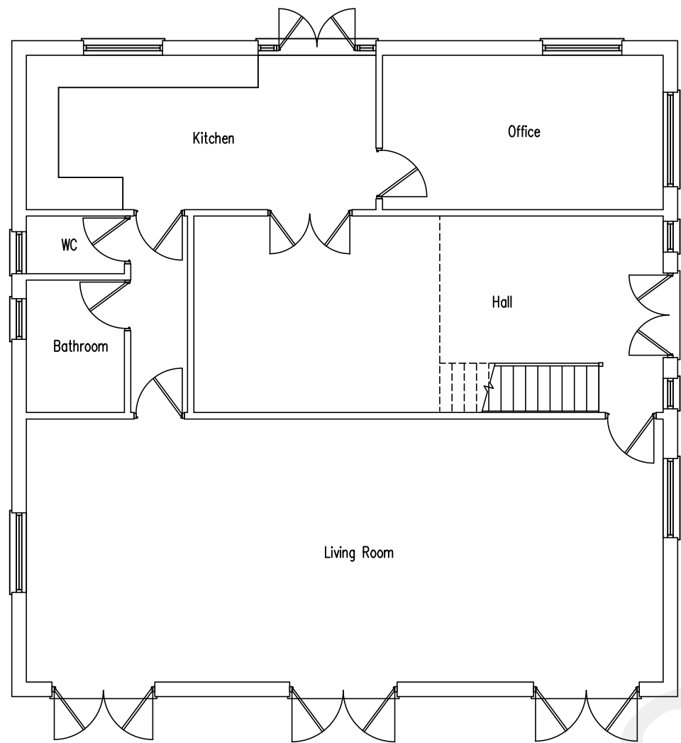
Existing Ground Floor Plan Scale 1:100 @ A1
