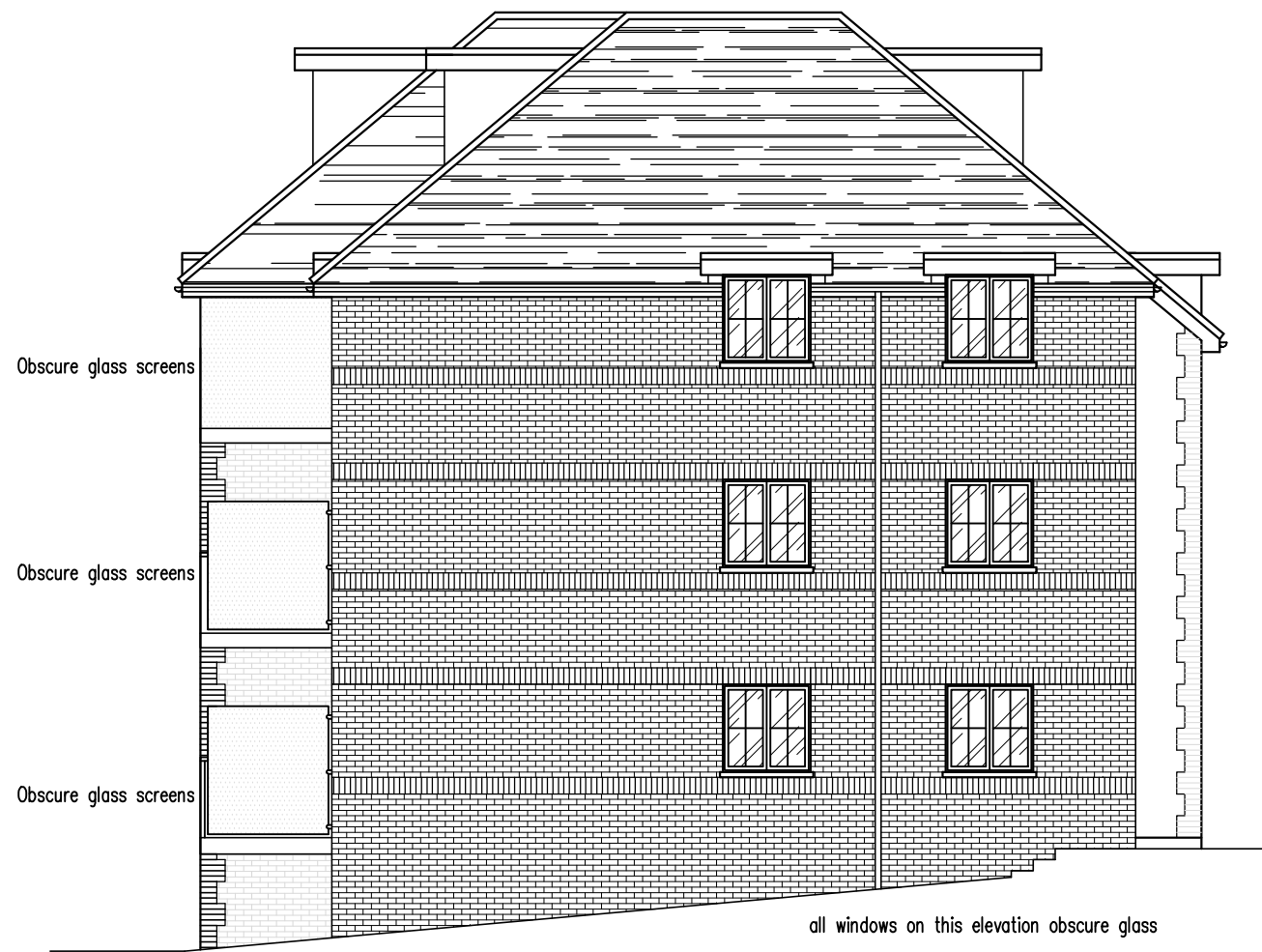
Proposed Side (West) Elevation Scale 1:100 @ A1
