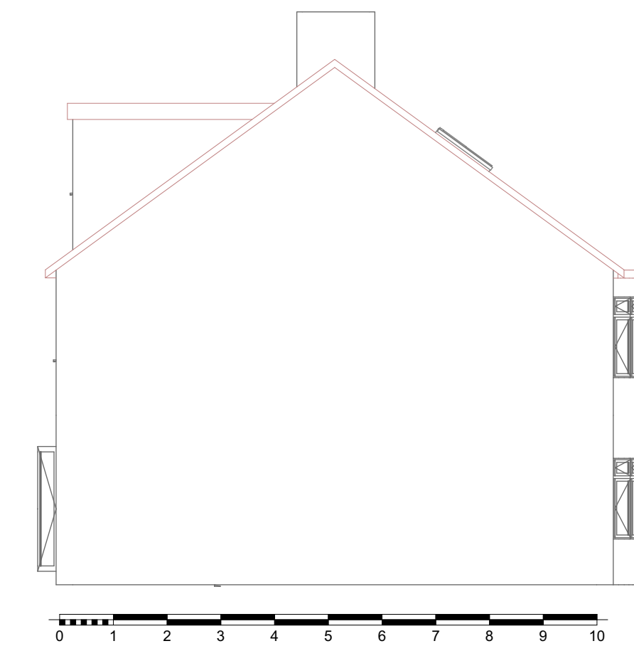
7 North Elevation Proposed 1:100
