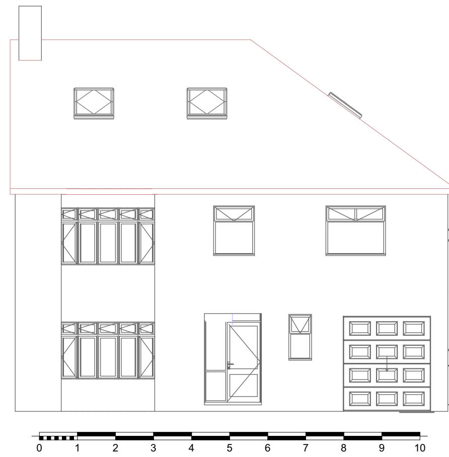
6 West Elevation Proposed 1:100
