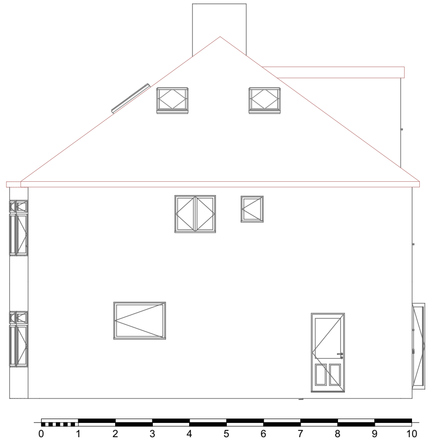
8 South Elevation Proposed 1:100
