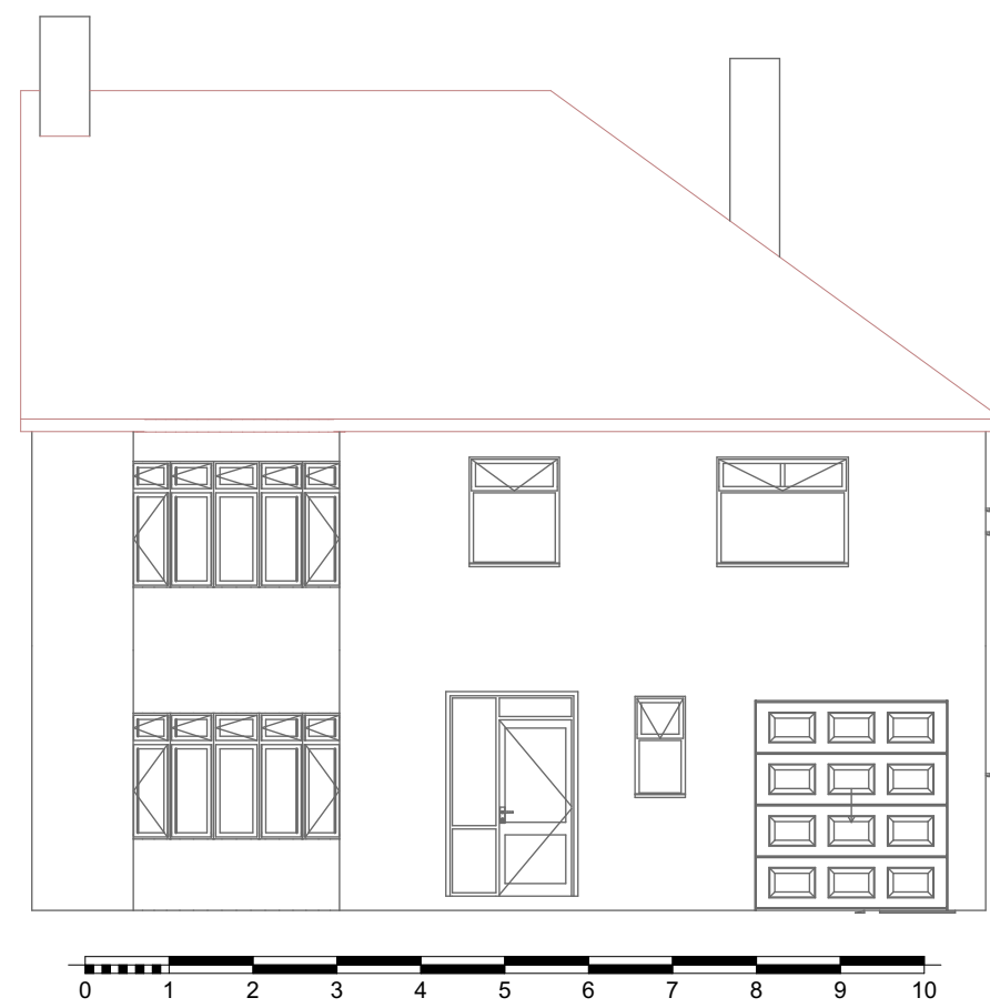
2 West Elevation Existing 1:100
