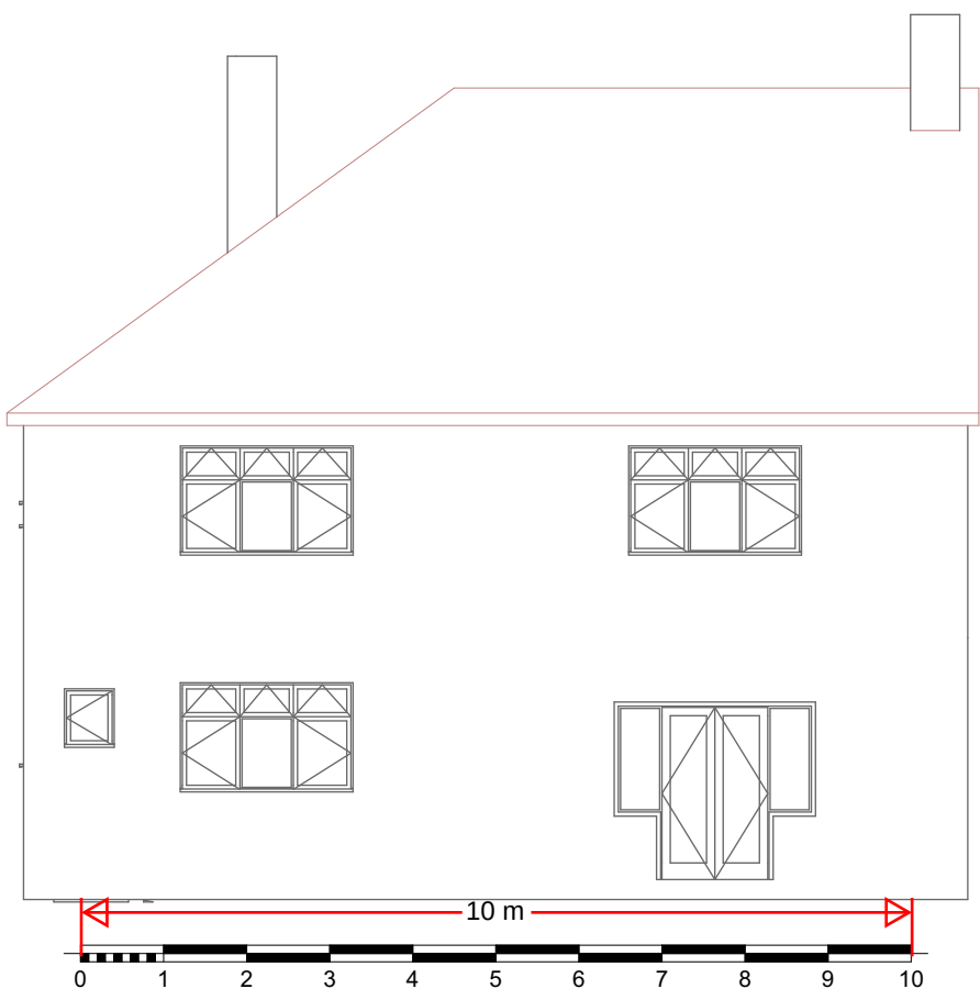
1 East Elevation Existing 1:100
