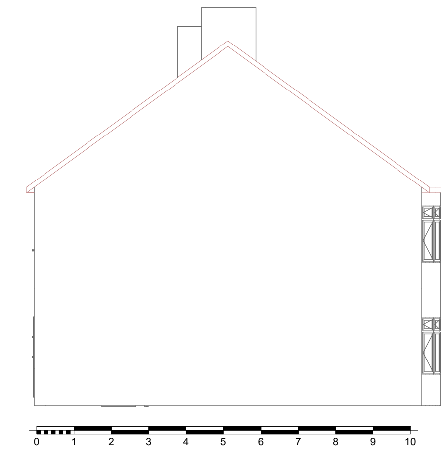
3 North Elevation Existing 1:100
