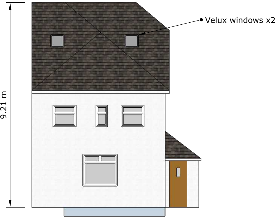
East Elevation
