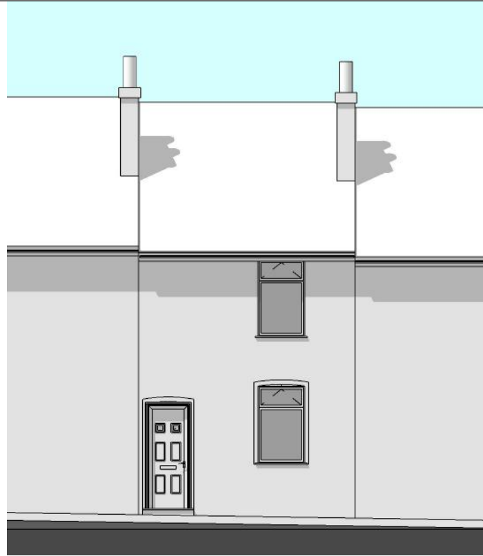
b front / east elevation 002 scale: 1:100 0 1 2m
