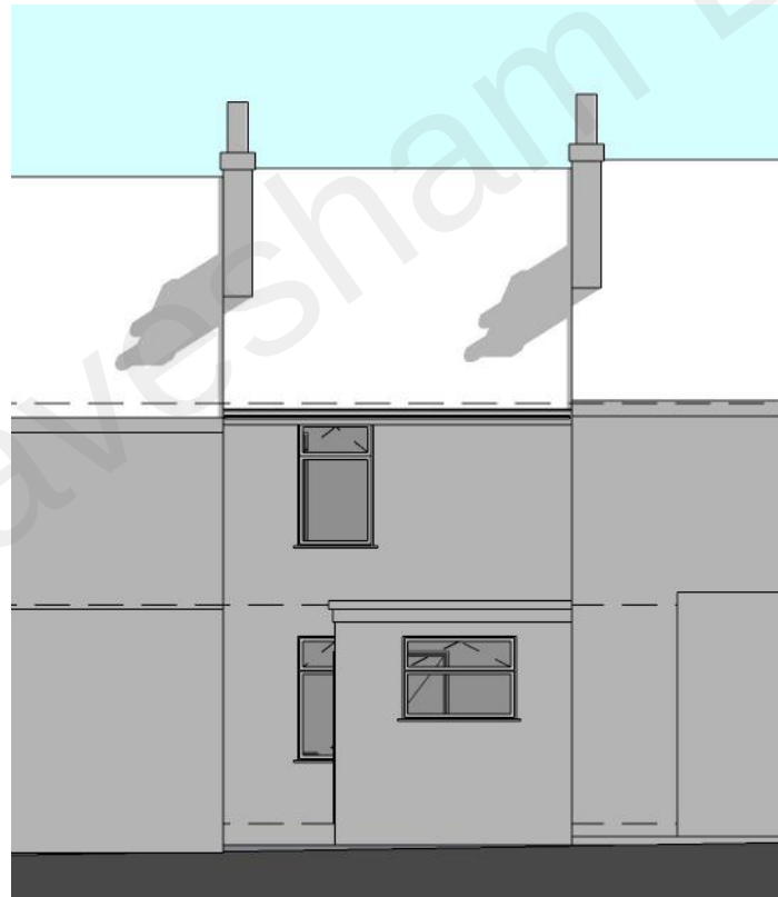
d garden / west elevation 004 scale: 1:100
