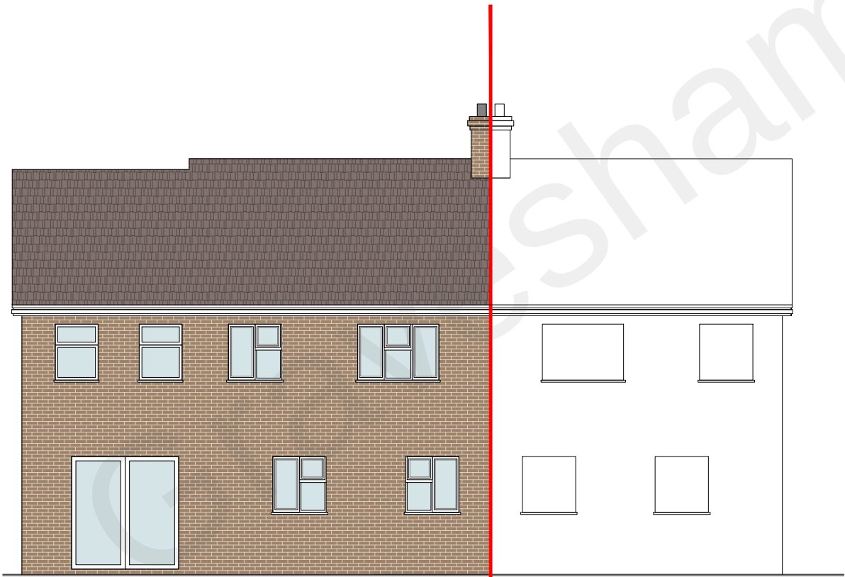
Rear (north) Elevation
