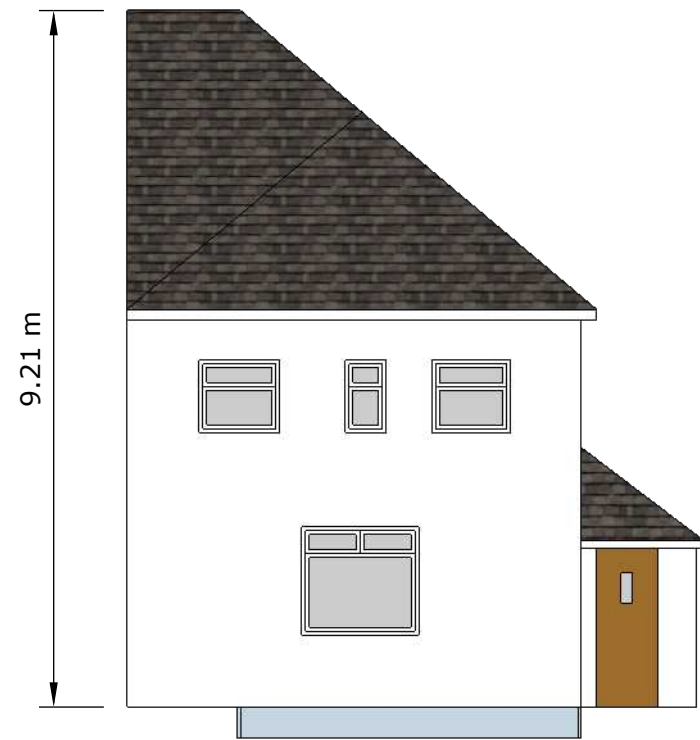
East Elevation
