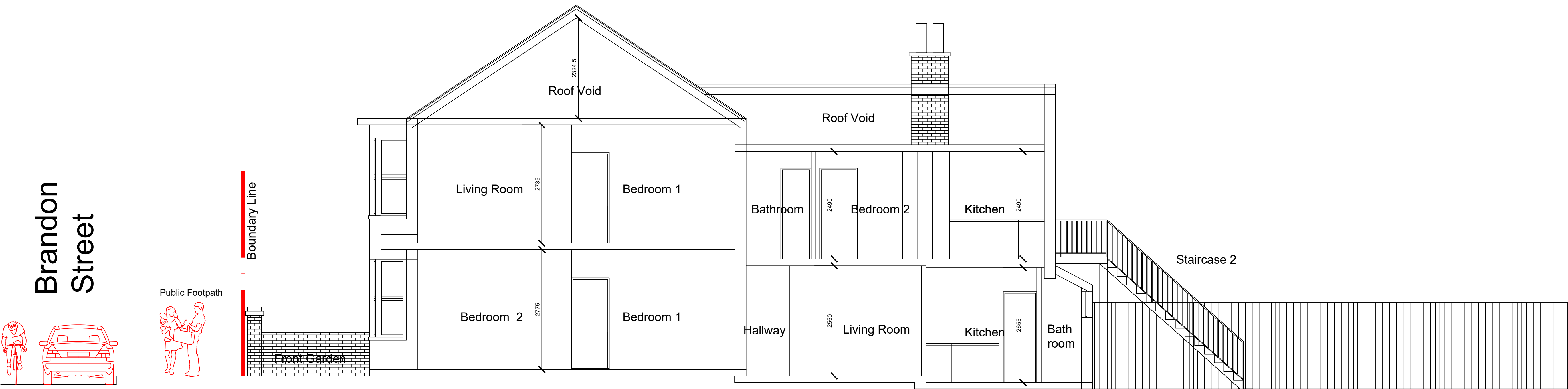
No 36 Brandon Street Proposed Section B-B
