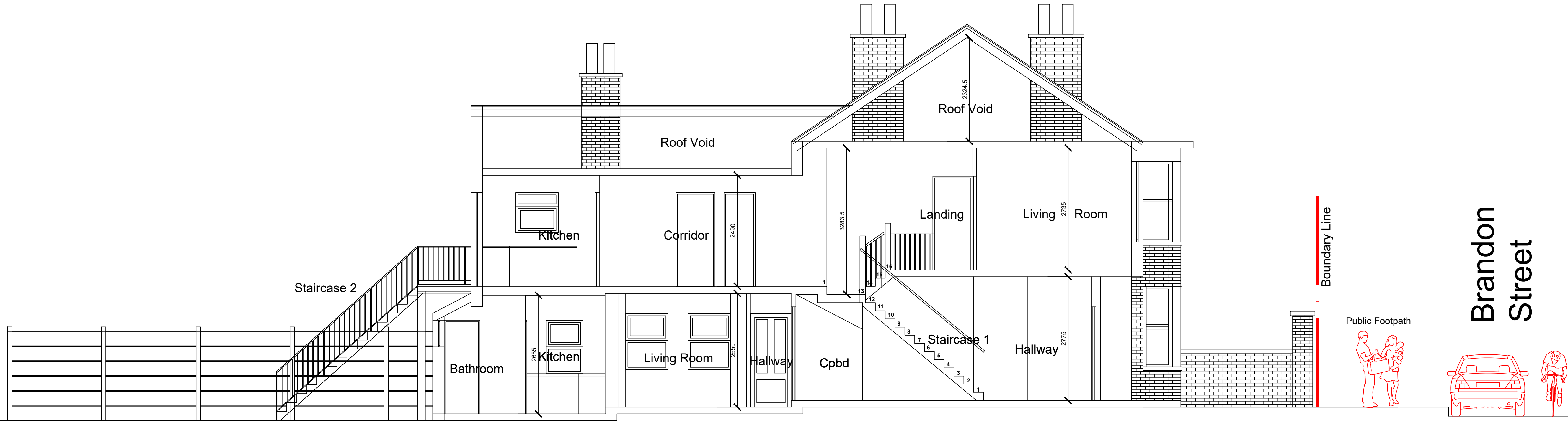
No 36 Brandon Street Proposed Section A-A
