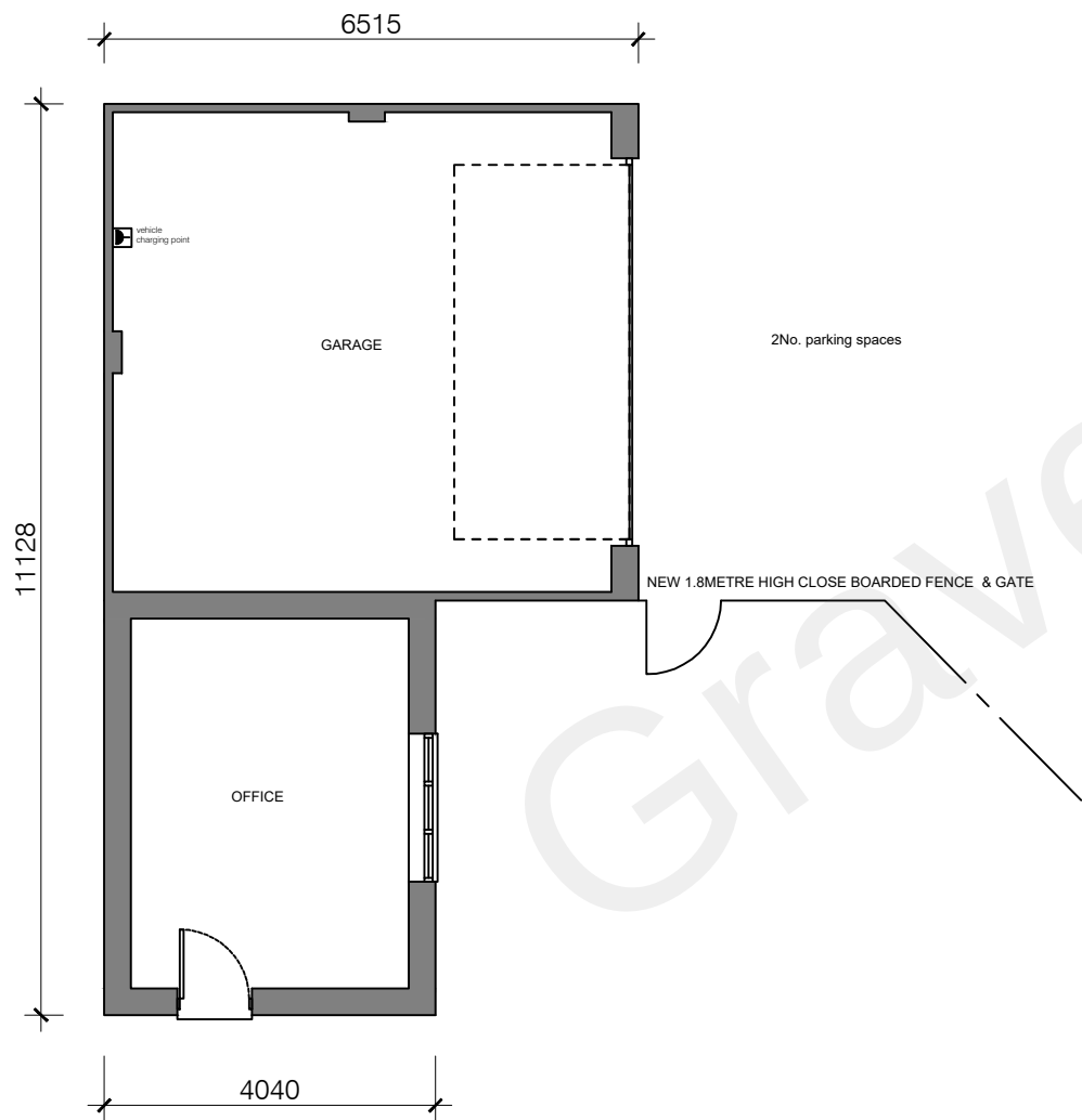
FLOOR PLAN 1:100
