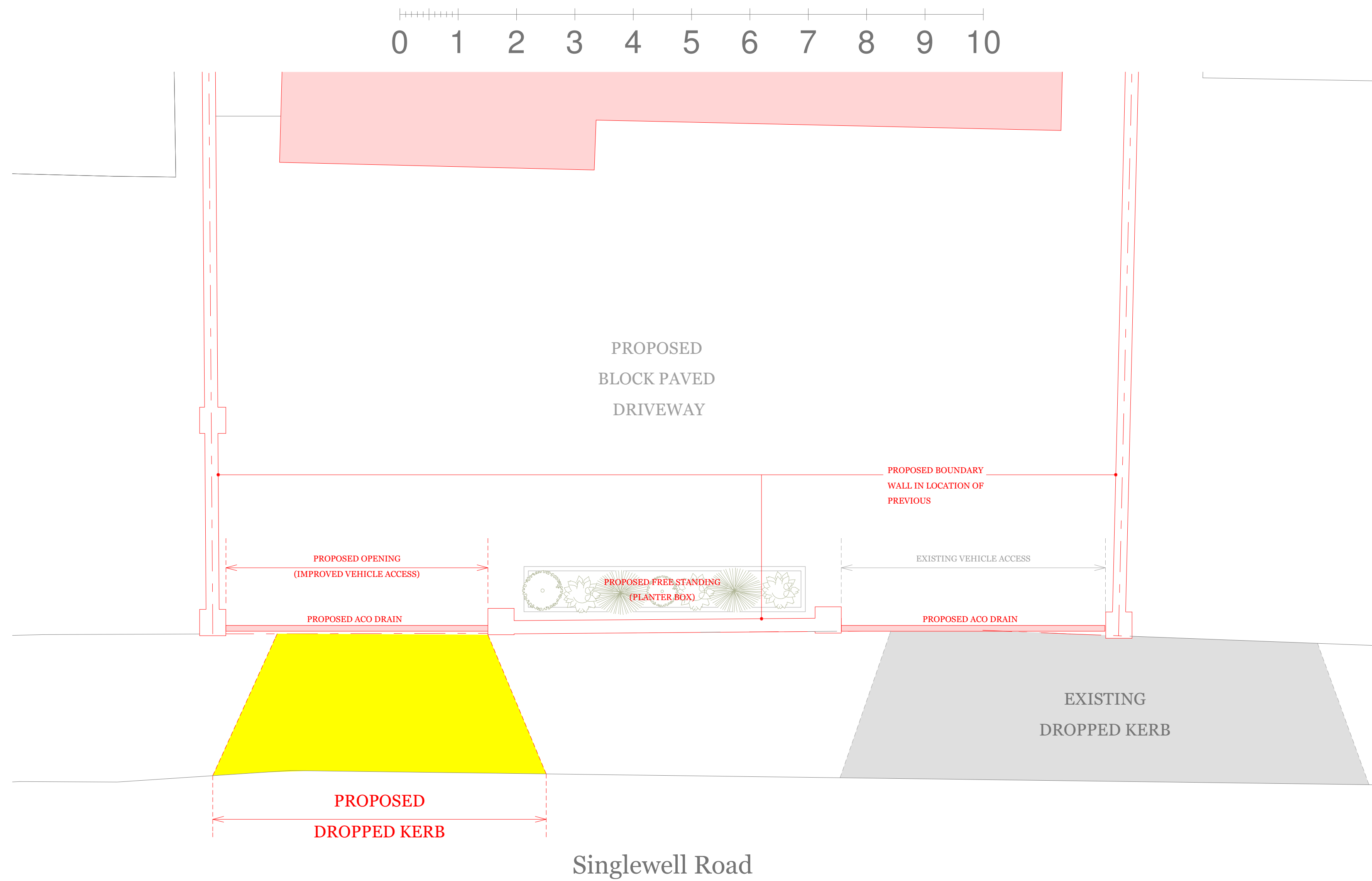
DRIVEWAY PLAN AS PROPOSED @ 1 : 50
