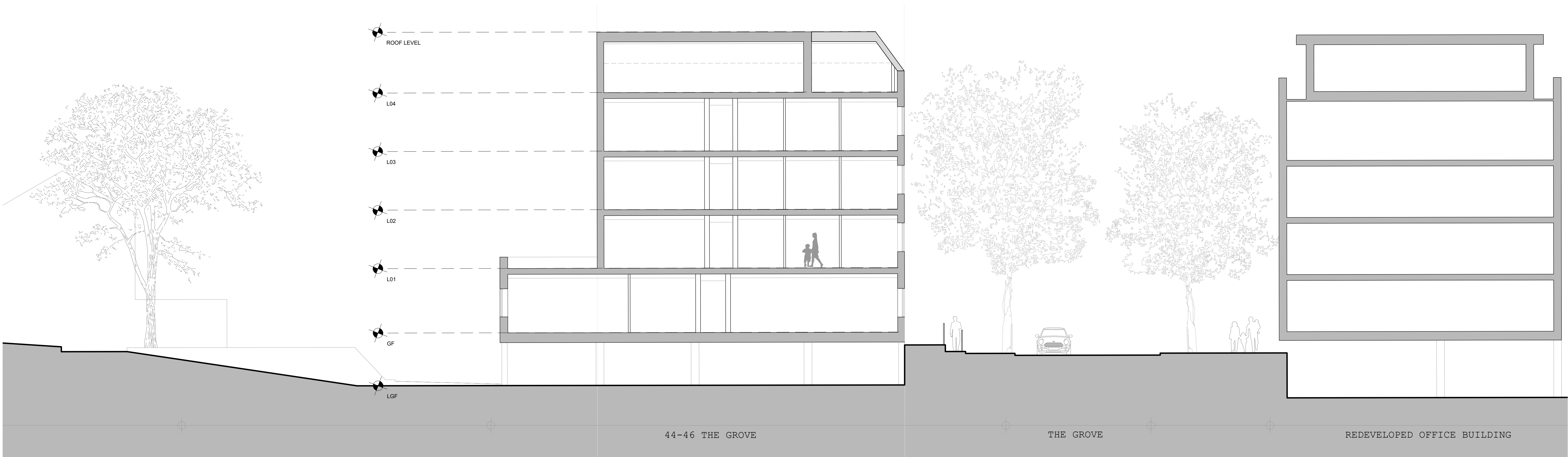
Proposed Section AA Scale 1:100 @ A1
