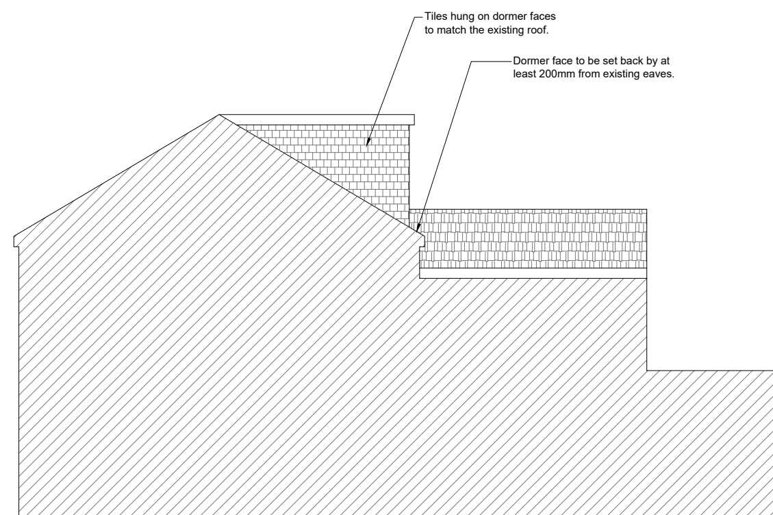
PROPOSED SIDE ELEVATION- 'B'
