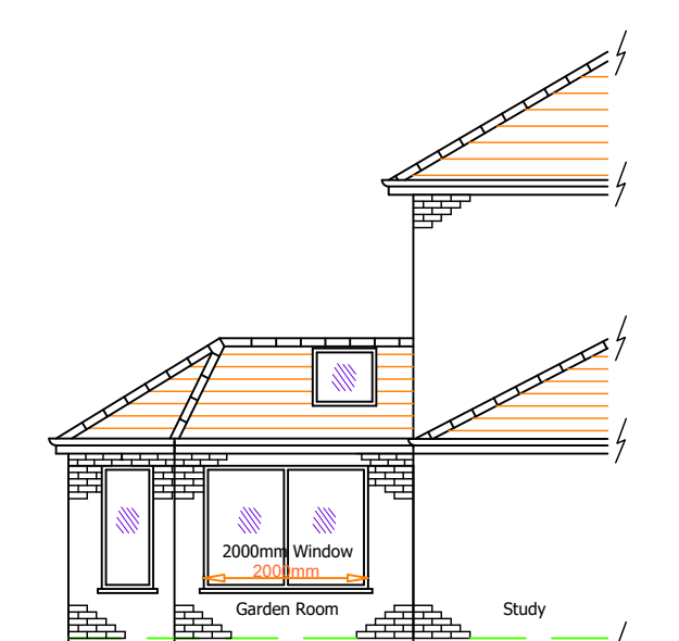
Proposed Side (East) Elevation 1:100
