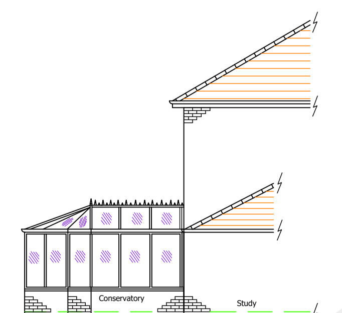
Existing Side (East) Elevation 1:100
