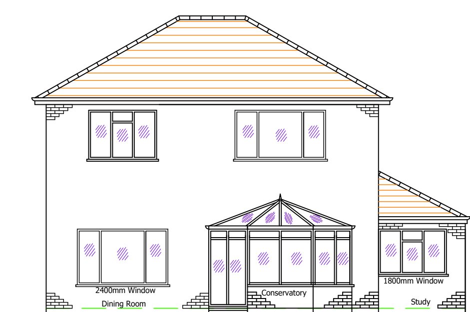
Existing Rear (South) Elevation 1:100
