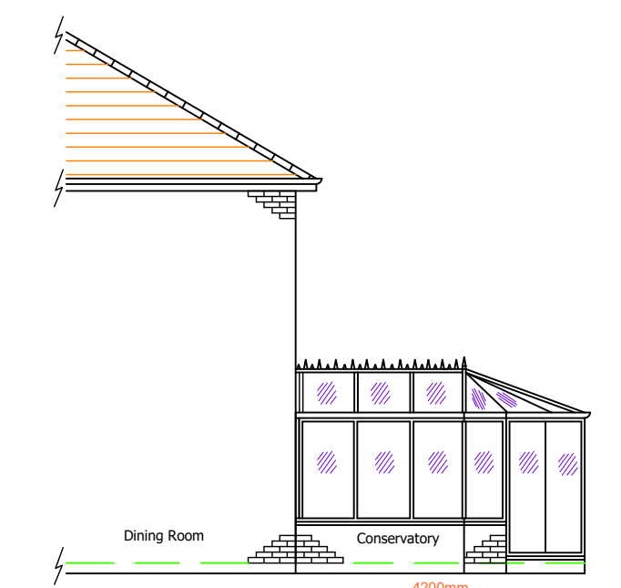
Existing Side (West) Elevation 1:100
