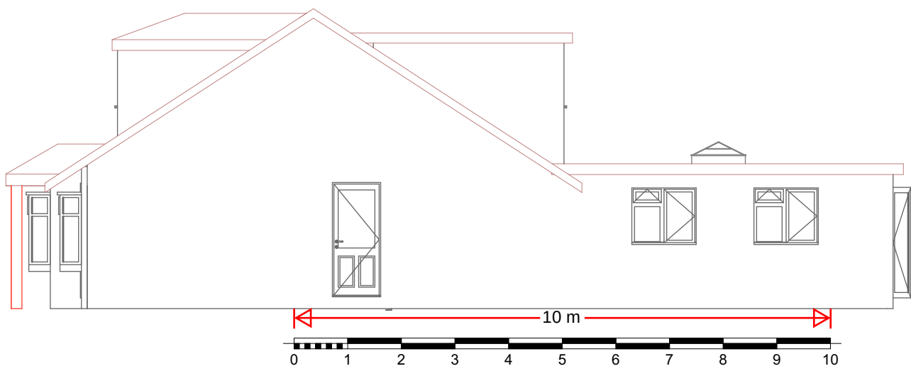
5 East Elevation Proposed 1:100
