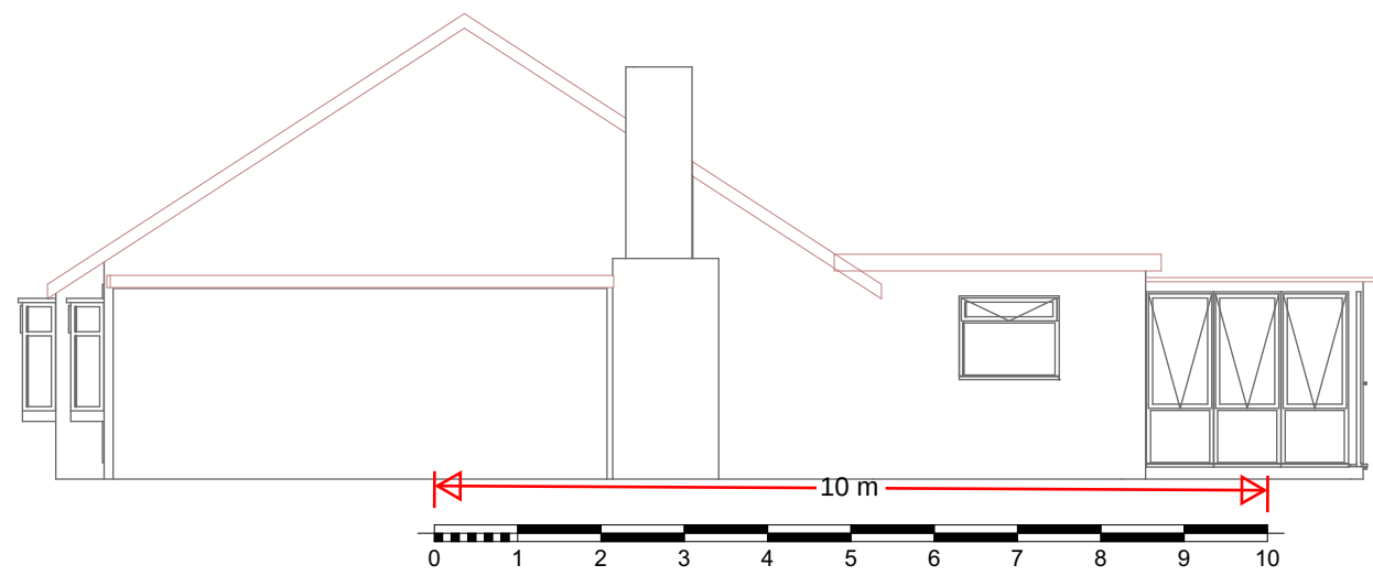
1 East Elevation Existing 1:100
