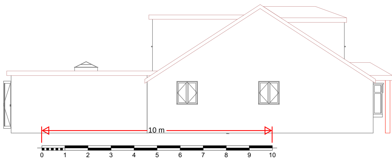
6 West Elevation Proposed 1:100
