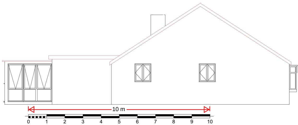
2 West Elevation Existing 1:100
