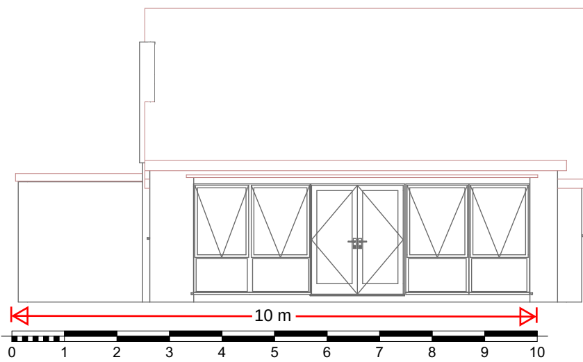
3 North Elevation Existing 1:100
