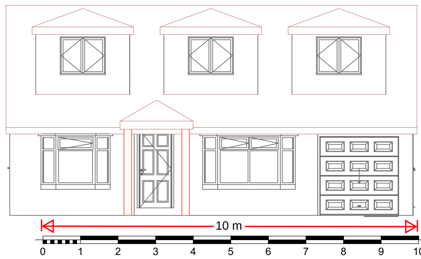
8 South Elevation Proposed 1:100
