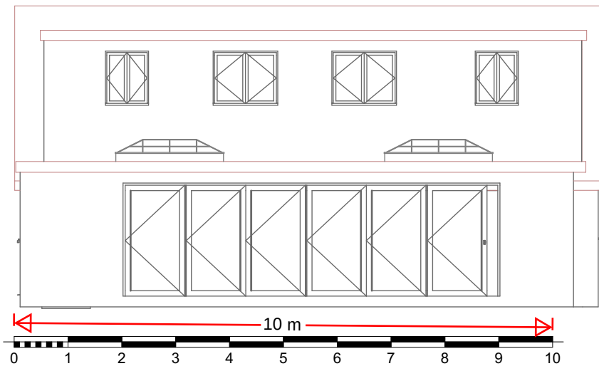
7 North Elevation Proposed 1:100
