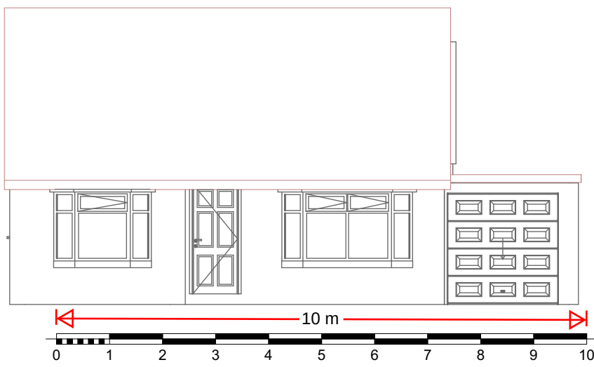
4 South Elevation Existing 1:100
