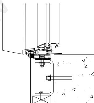
Windoor System 1000, cill detail
