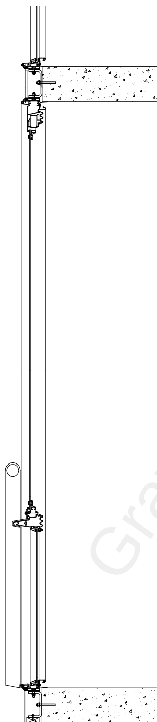
Windoor System 1000, vertical section
