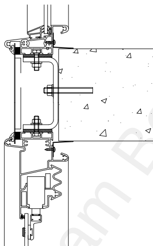
Windoor System 1000, head/intermediate detail
