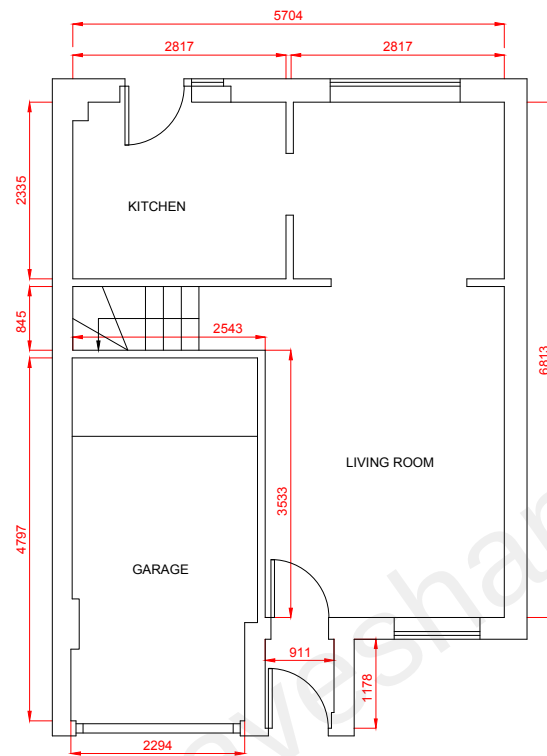
EXISTING GROUND FLOOR
