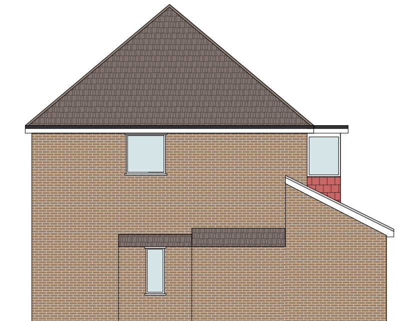
Proposed Side Elevation (South)
