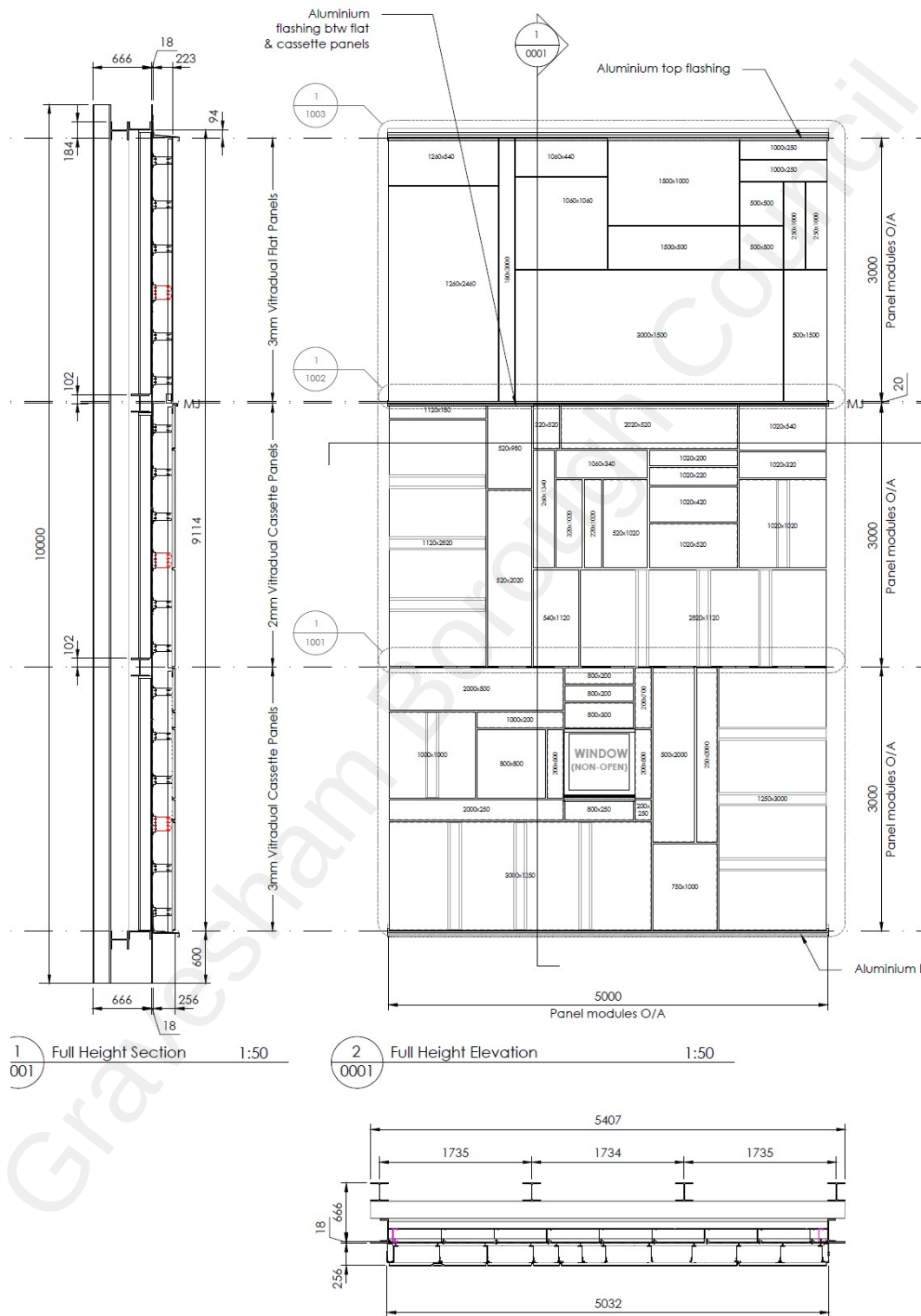
Elevation and sections of wall showing arrangement of panels
