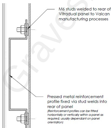
Stiffener attachment detail
