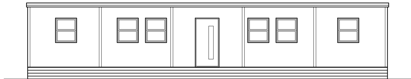
Block 4 - Existing front elevation @ 1:100
