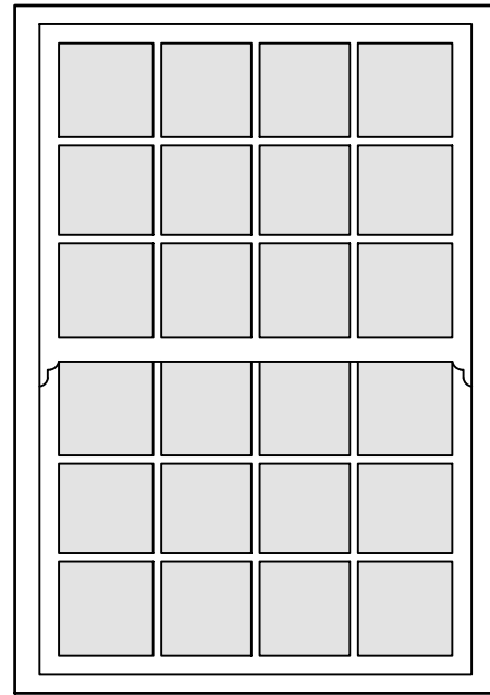
Pre-existing Windows 1:20
