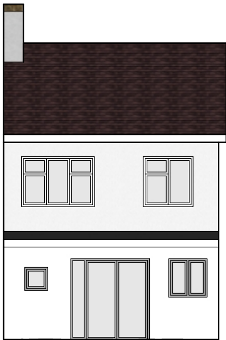
East Elevation
