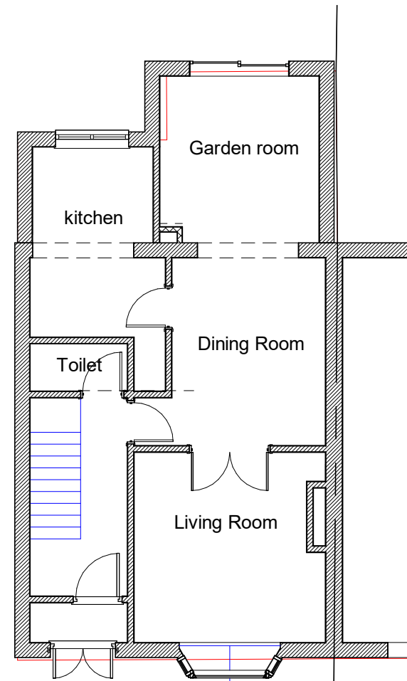
0 Ex Ground Floor 1 : 100
