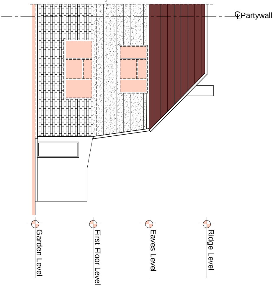
Pre Existing Rear Elevation
