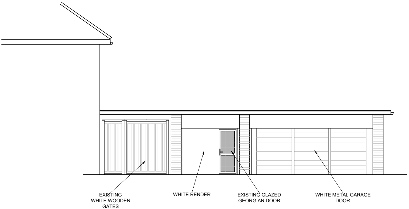
SOUTH ELEVATION
