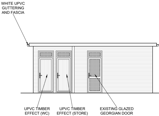
WEST ELEVATION
