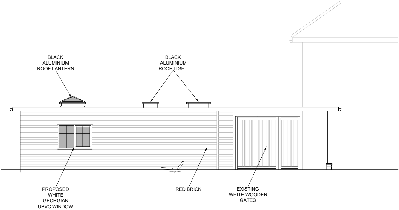
NORTH ELEVATION
