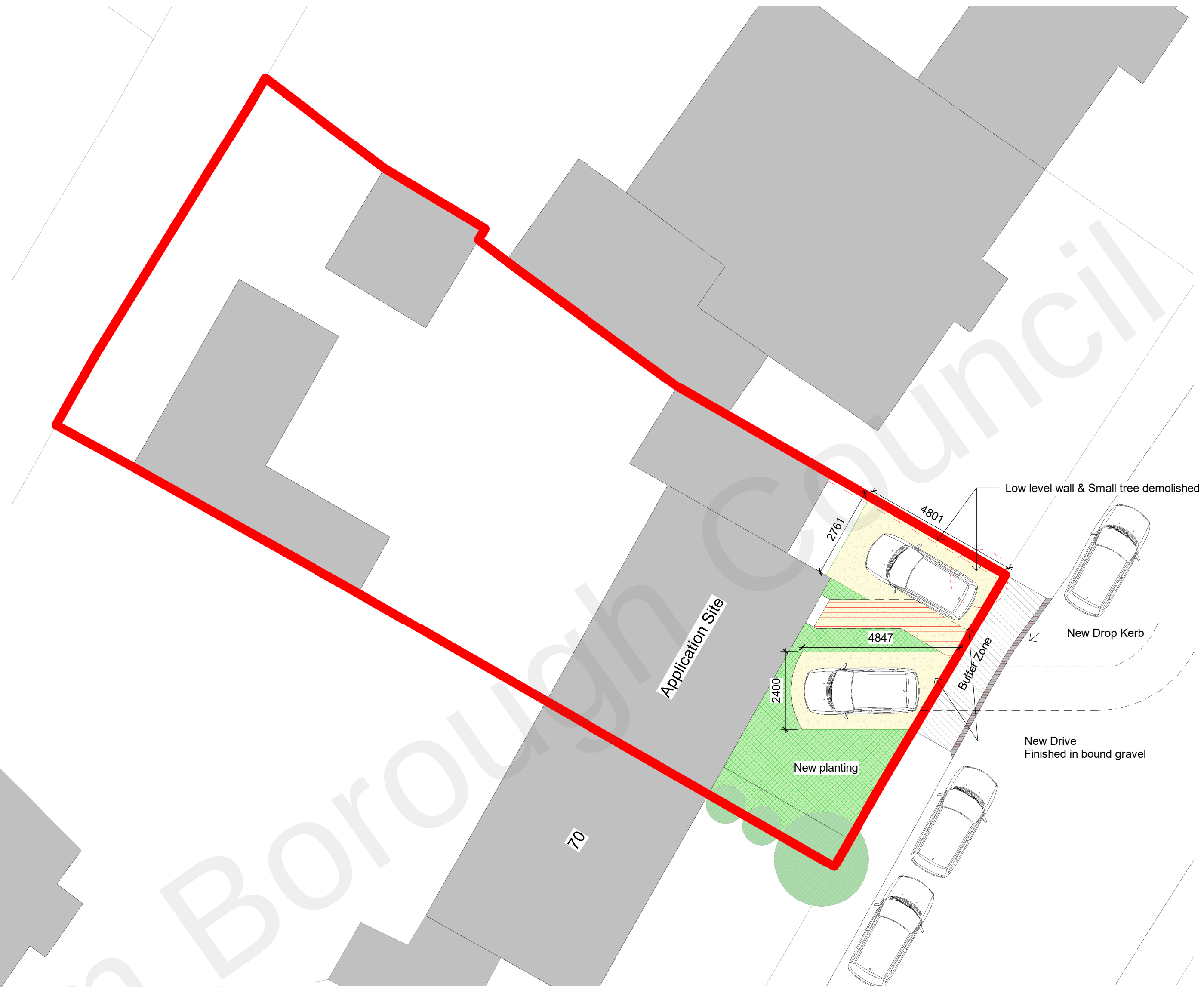
3 Proposed Plan 1 : 100
