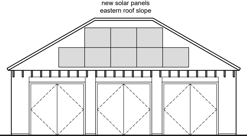
FRONT ELEVATION
