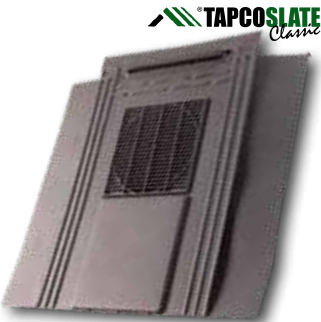
Classic Slate Inline Vent 10,000mm²/m Ventilation
