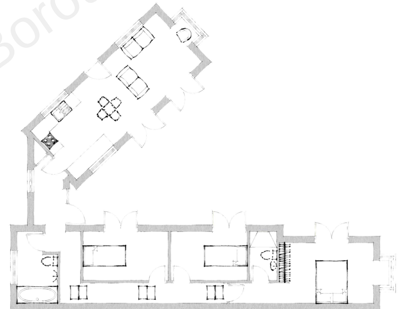
Floor Plan
