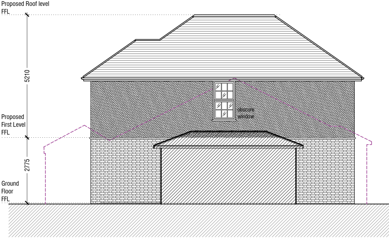
PROPOSED SIDE ELEVATION E4 Scale 1:100
