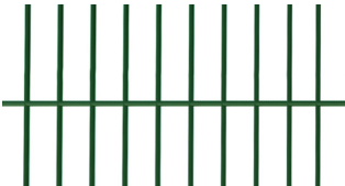
ZedPanel V-Mesh Green • 4mm Vertical Wire / 5mm Horizontal Wire/ 200mm x 50mm Aperture Size • Colour Coated Wire Green
