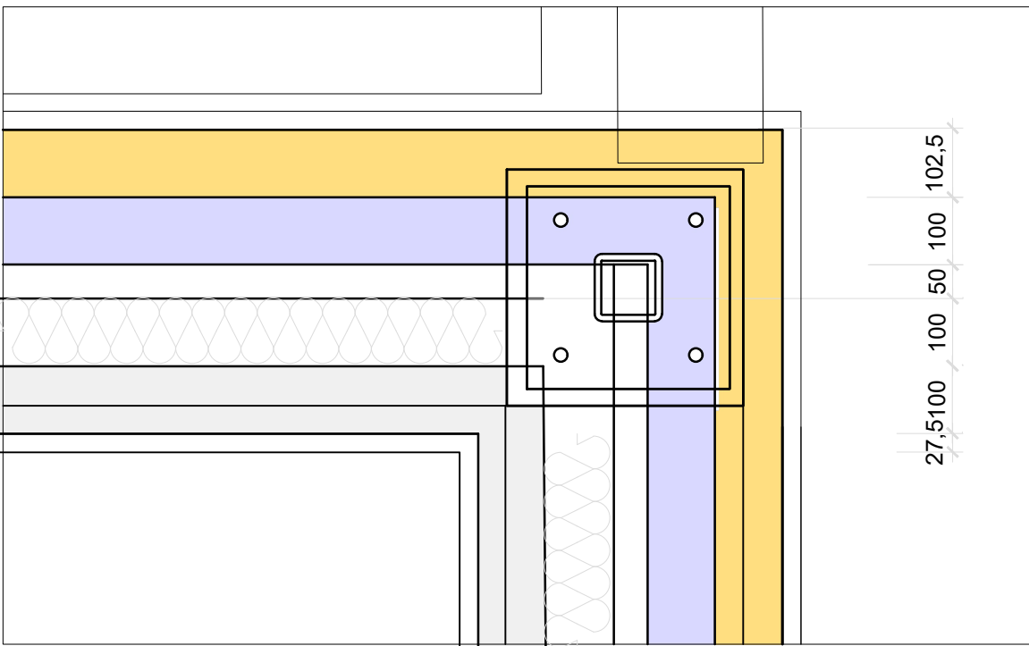
DETAIL 3
