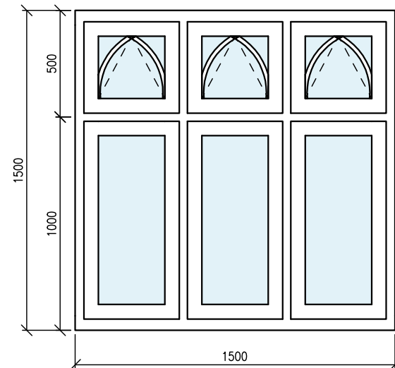
Window - W1 Flush Casement
