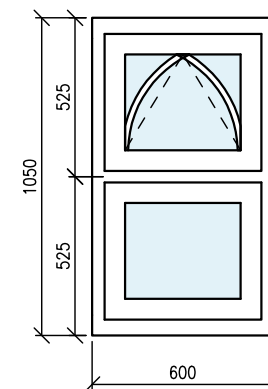
Window - W2 Flush Casement
