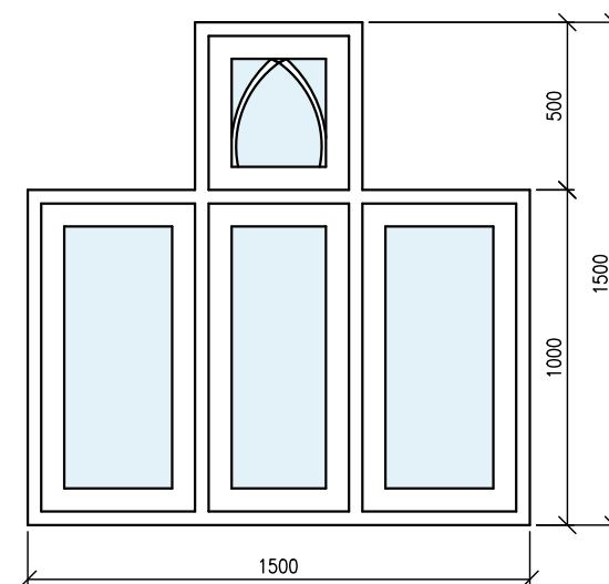
Window - W6 Flush Casement
