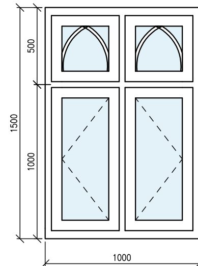
Window - W4, W5, W8, W9, W10 Flush Casement
