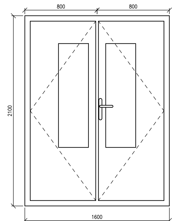
Door - D1 Casement French Door
