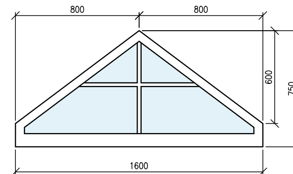
Window - W7 Flush Casement
