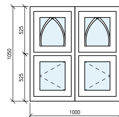
Window - W3 Flush Casement
