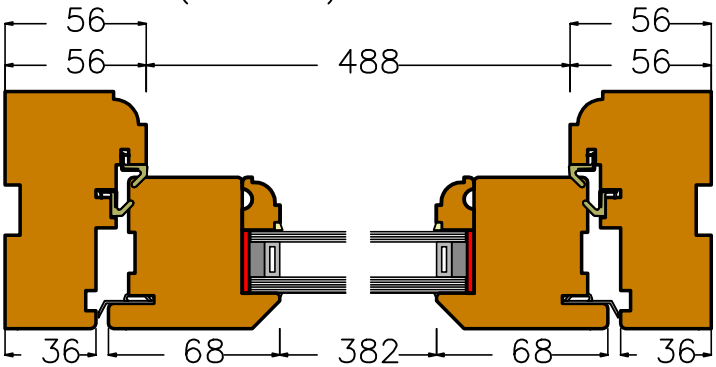
Section C2 (scale 1:3)
