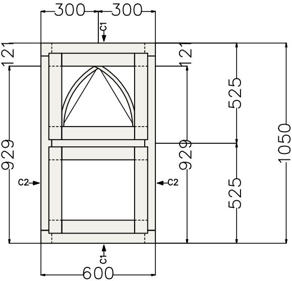
View from outside (scale 1:20)
