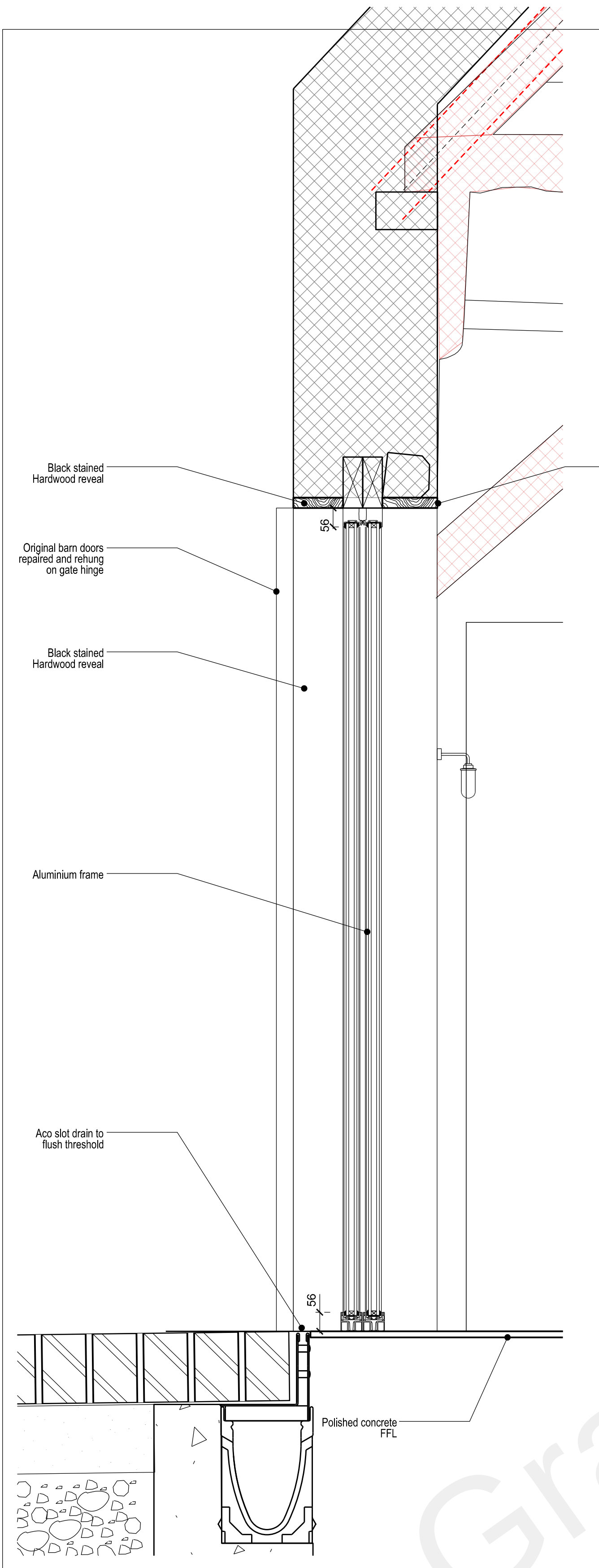
DETAIL - GF.W.01
