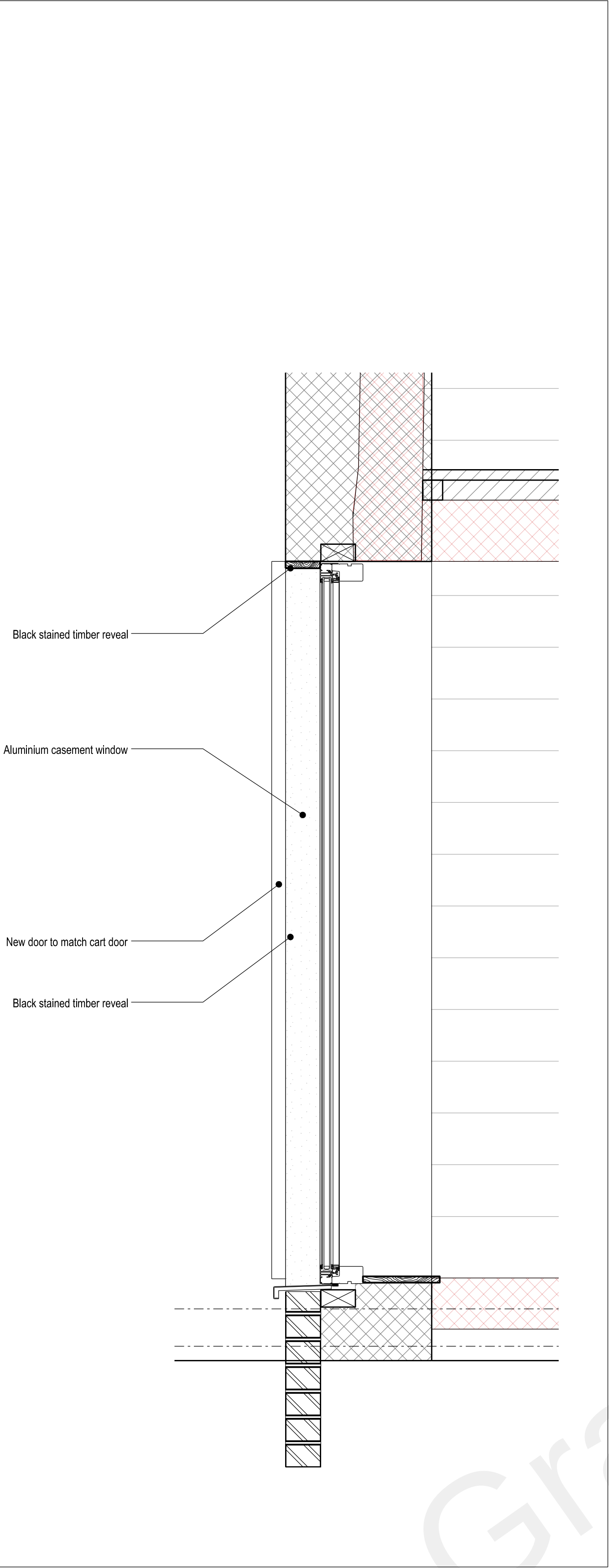
01 SECTION DETAIL
