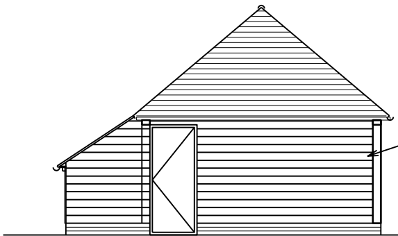
SIDE ELEVATION TO HOUSE
