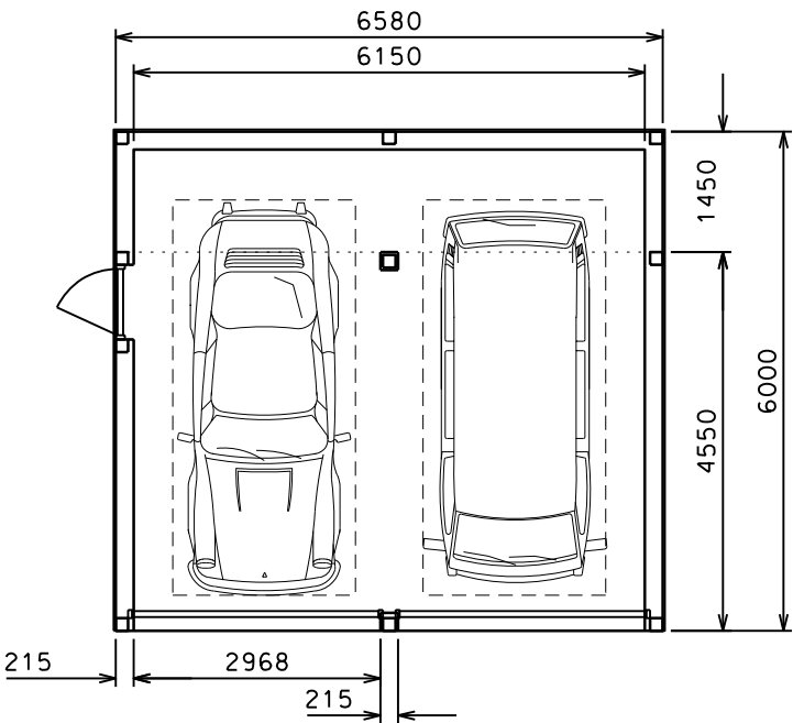
FLOOR PLAN
