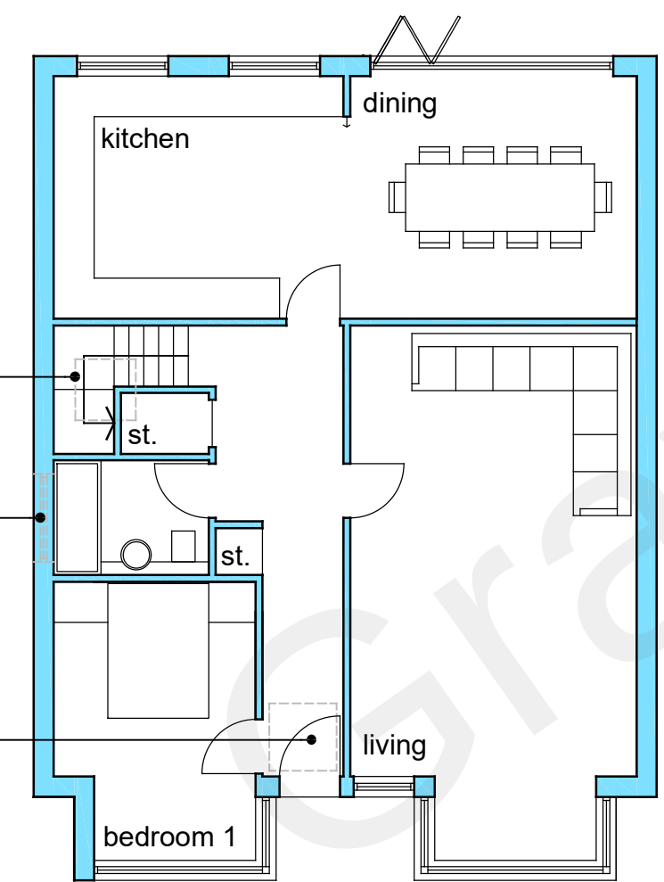
ground plan plot 1 4 bedroom, 7 person house, GIA 150sqm
