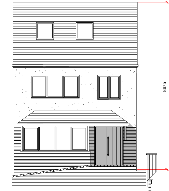
West Elevation
