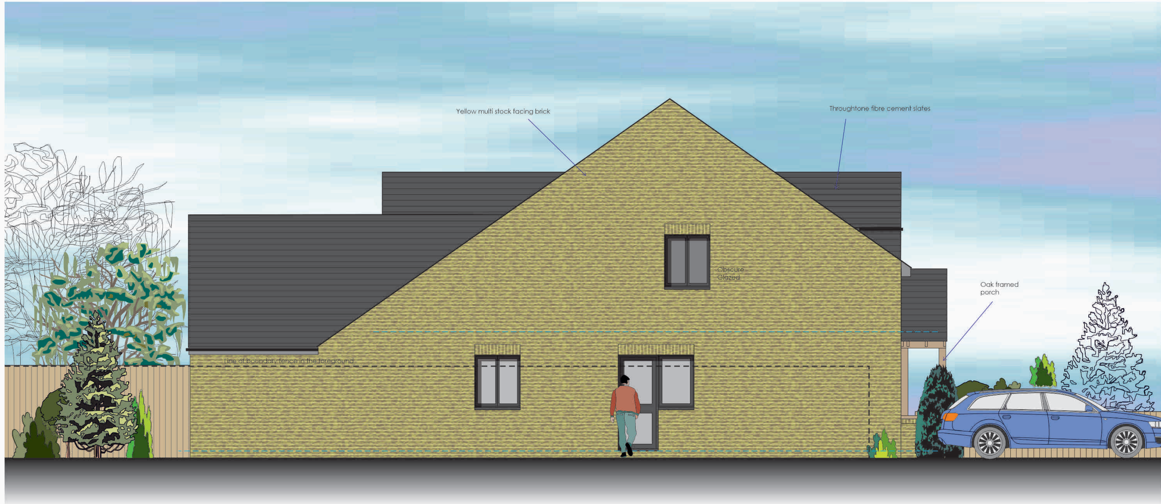
Proposed Side Elevation - 1:50 View from No 32
