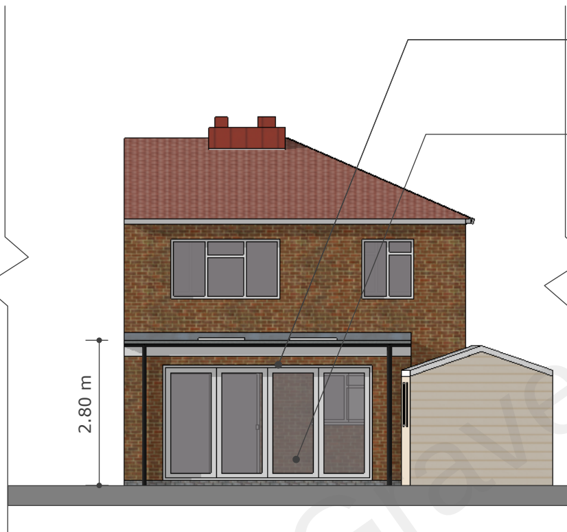
PROPOSED ELEVATION C-C SCALE 1:100 @ A3
