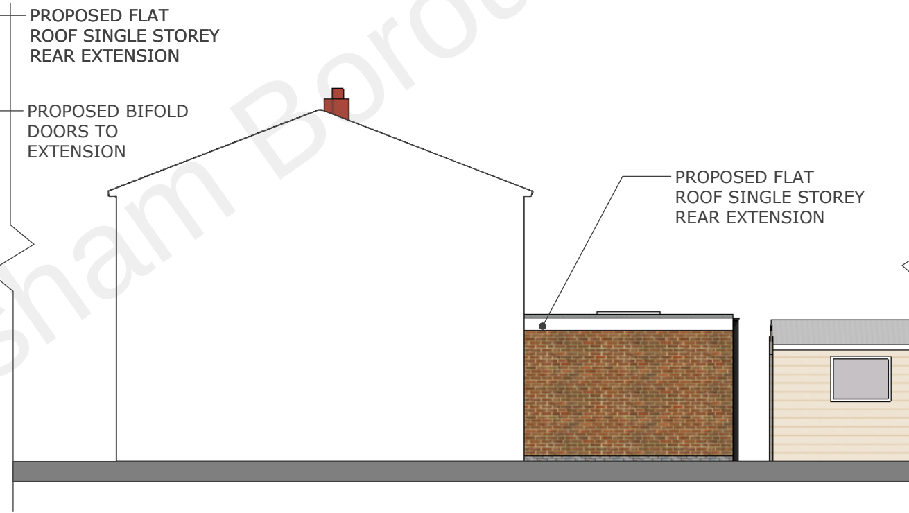
PROPOSED ELEVATION D-D SCALE 1:100 @ A3
