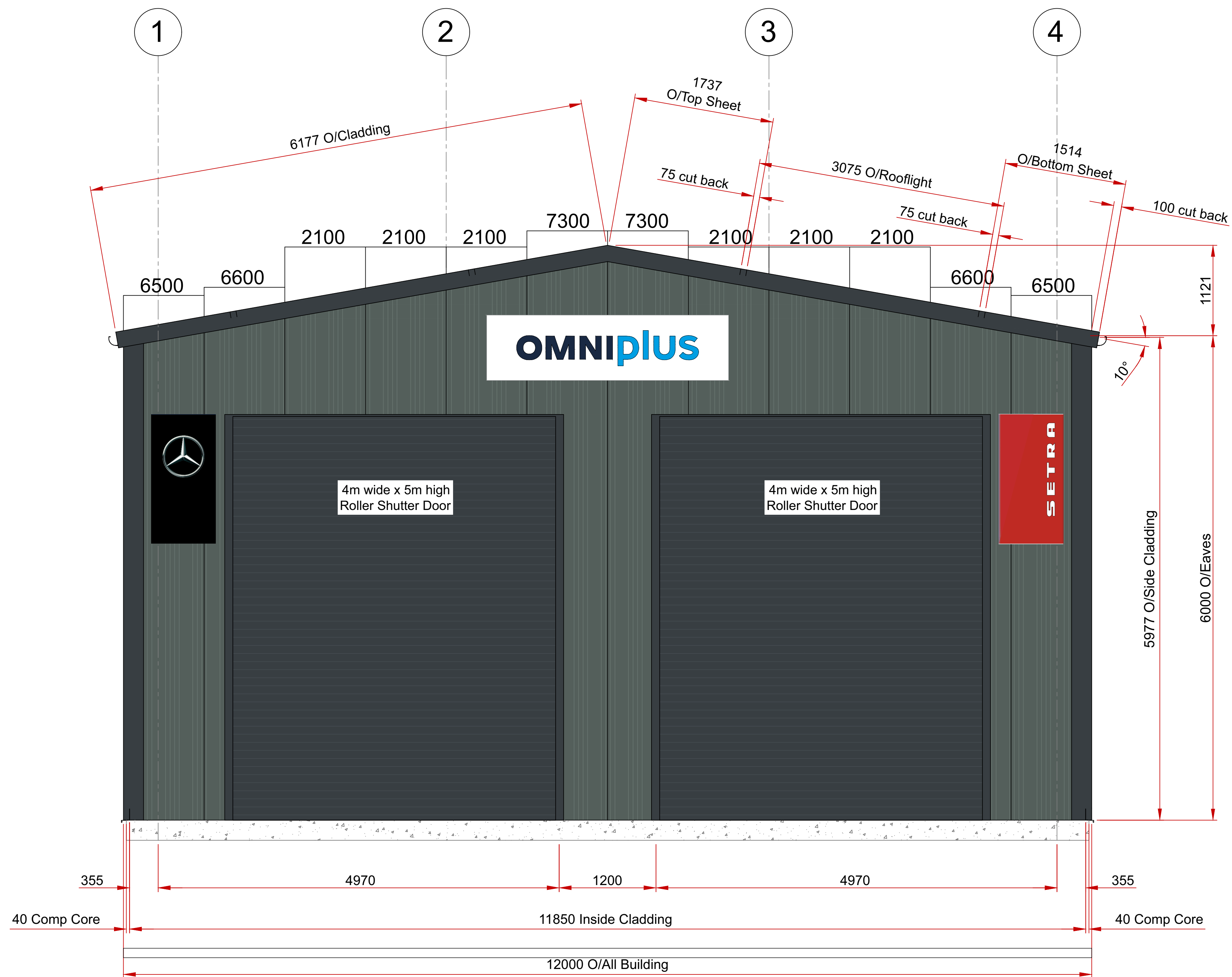
FRONT GABLE ELEVATION - SHEETING LAYOUT Cladding colour - Merlin Grey (BS 18B25) Flashings colour - Anthracite (RAL 7016)
