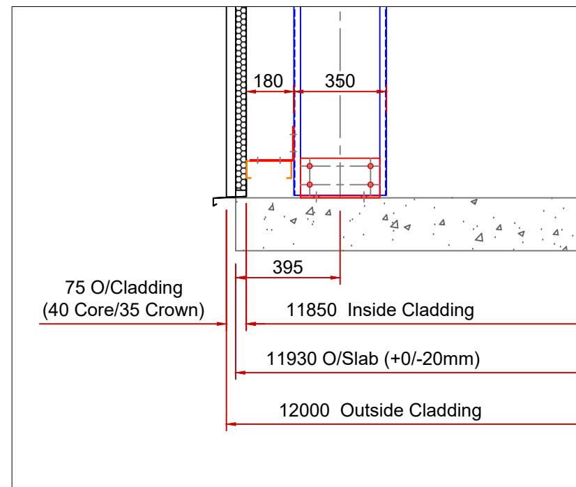
Enlarged Section Thru Slab
