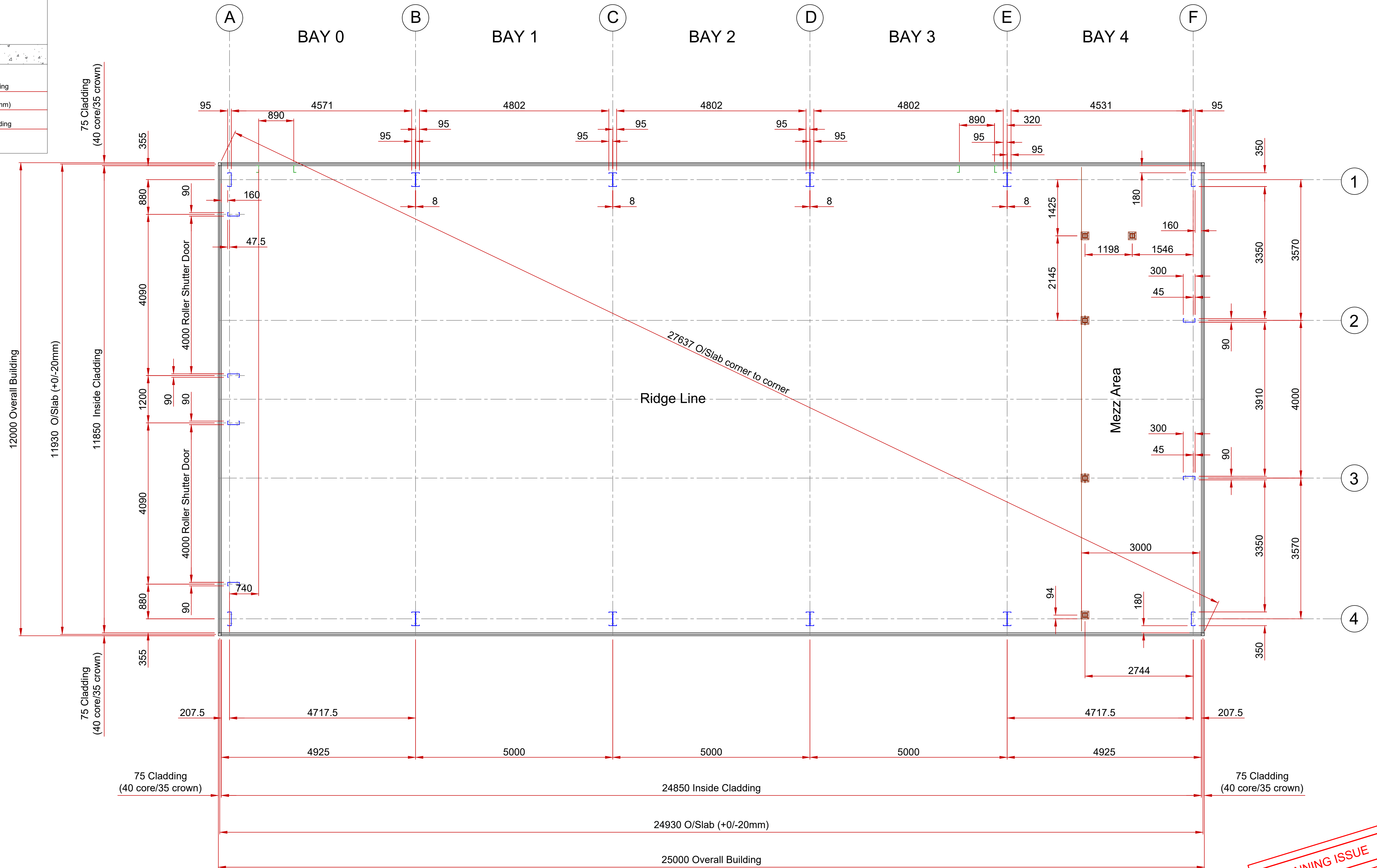
GRID-LINE PLAN (BASE LAYOUT)
