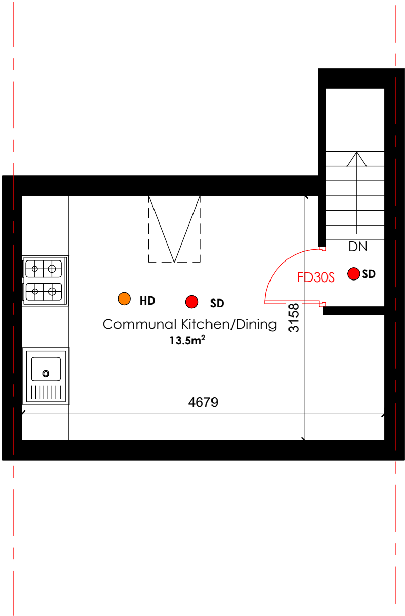
Proposed Loft Plan 1 : 50
