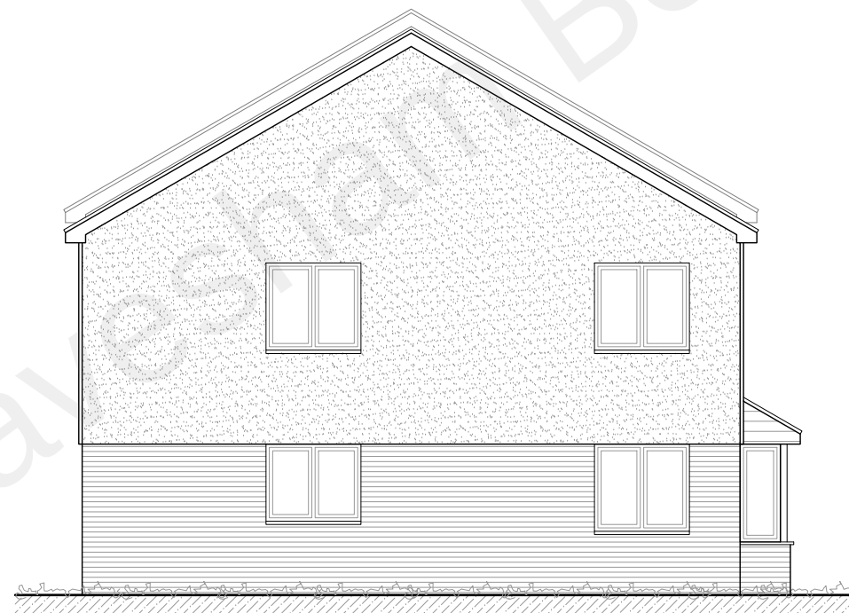
Side (south-facing) Elevation 1:100
