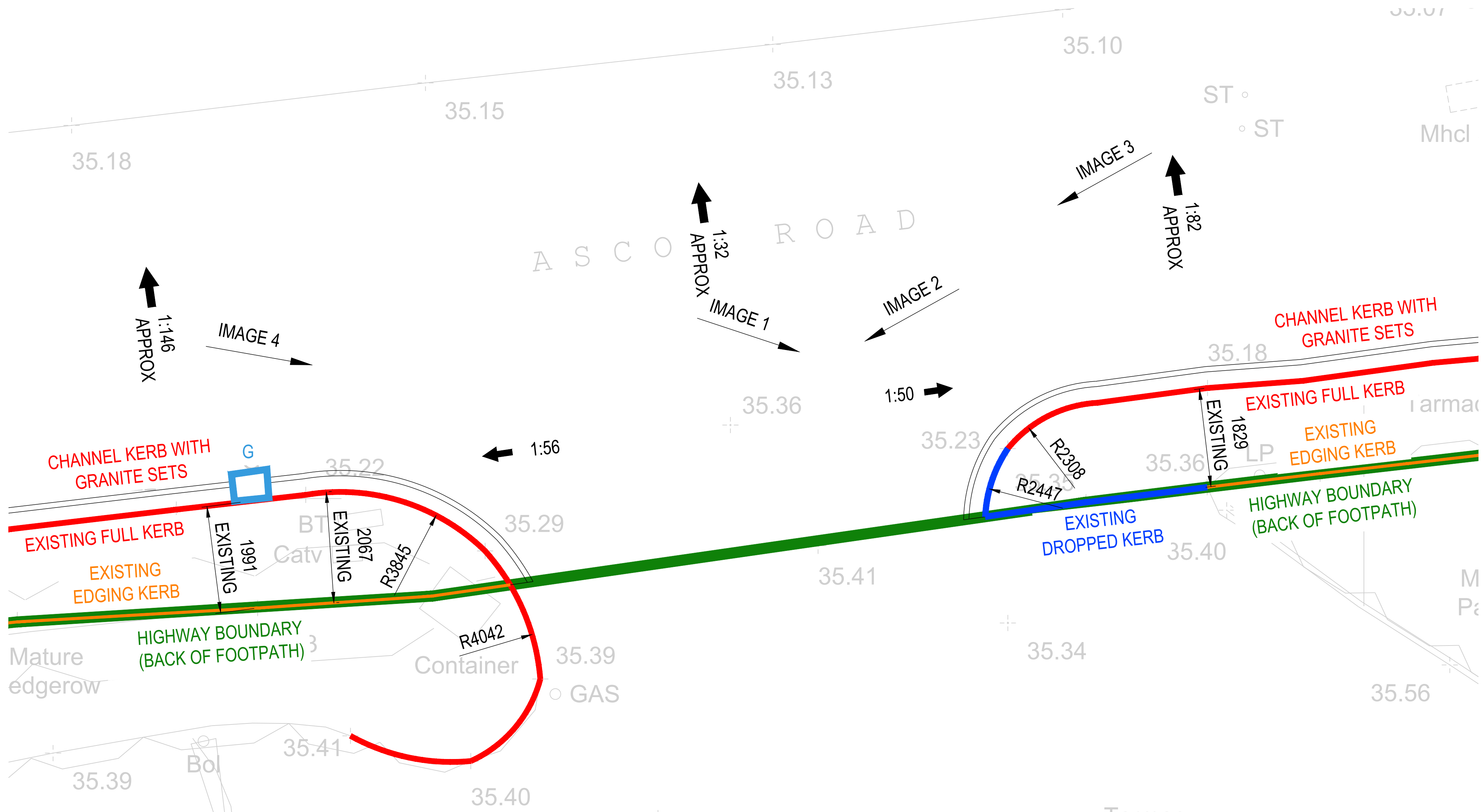
ASCOT ROAD EXISTING BELL MOUTH SCALE 1:50
