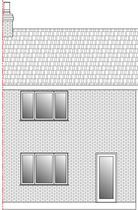
PRE-EXISTING FRONT ELEVATION
