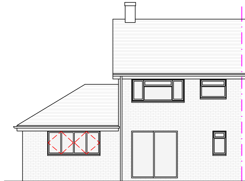
PROPOSED REAR (East) ELEVATION
