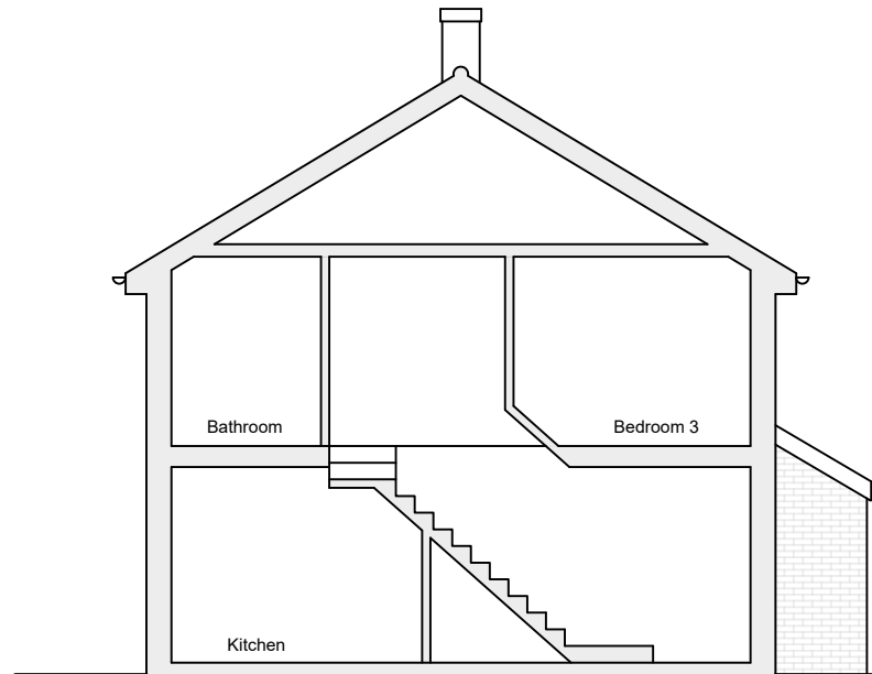
PROPOSED SIDE (North) ELEVATION / SECTION
